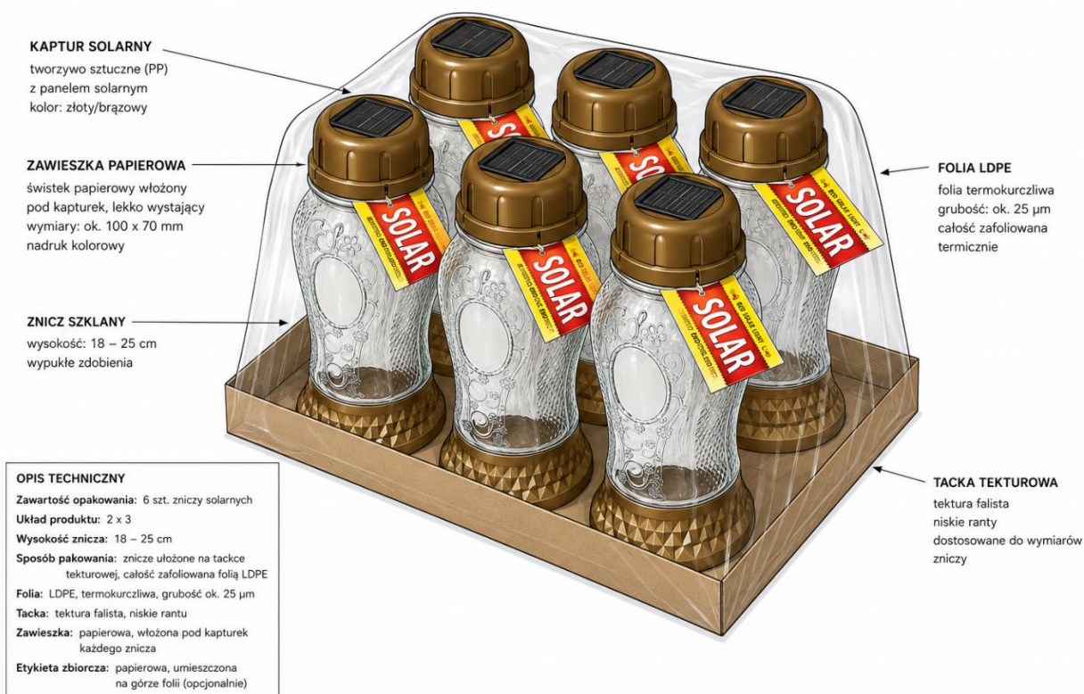
Figure 1. Illustrative configuration of the collective packaging for candles
