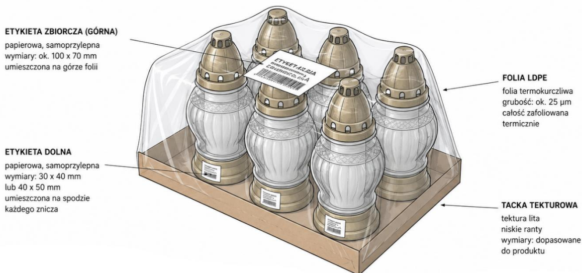
Figure 1. Illustrative configuration of the collective packaging for candles
